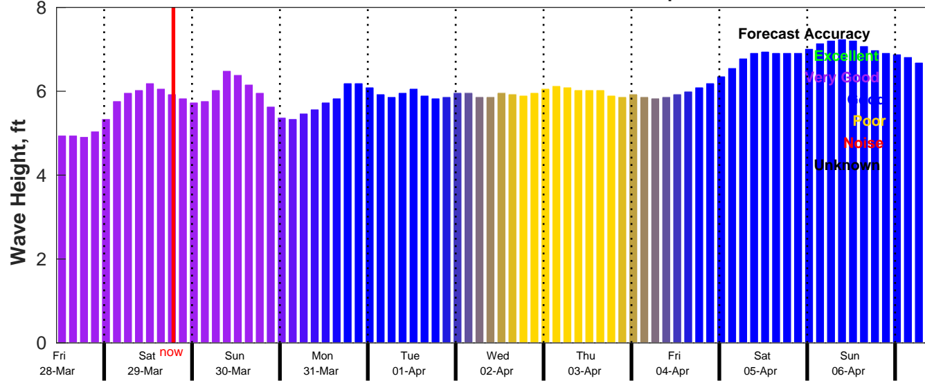
CMEMS Wave Forecast for NDBC 52213 from 27-Mar-2025 11:00:00 to 06-Apr-2025 11:00:00
