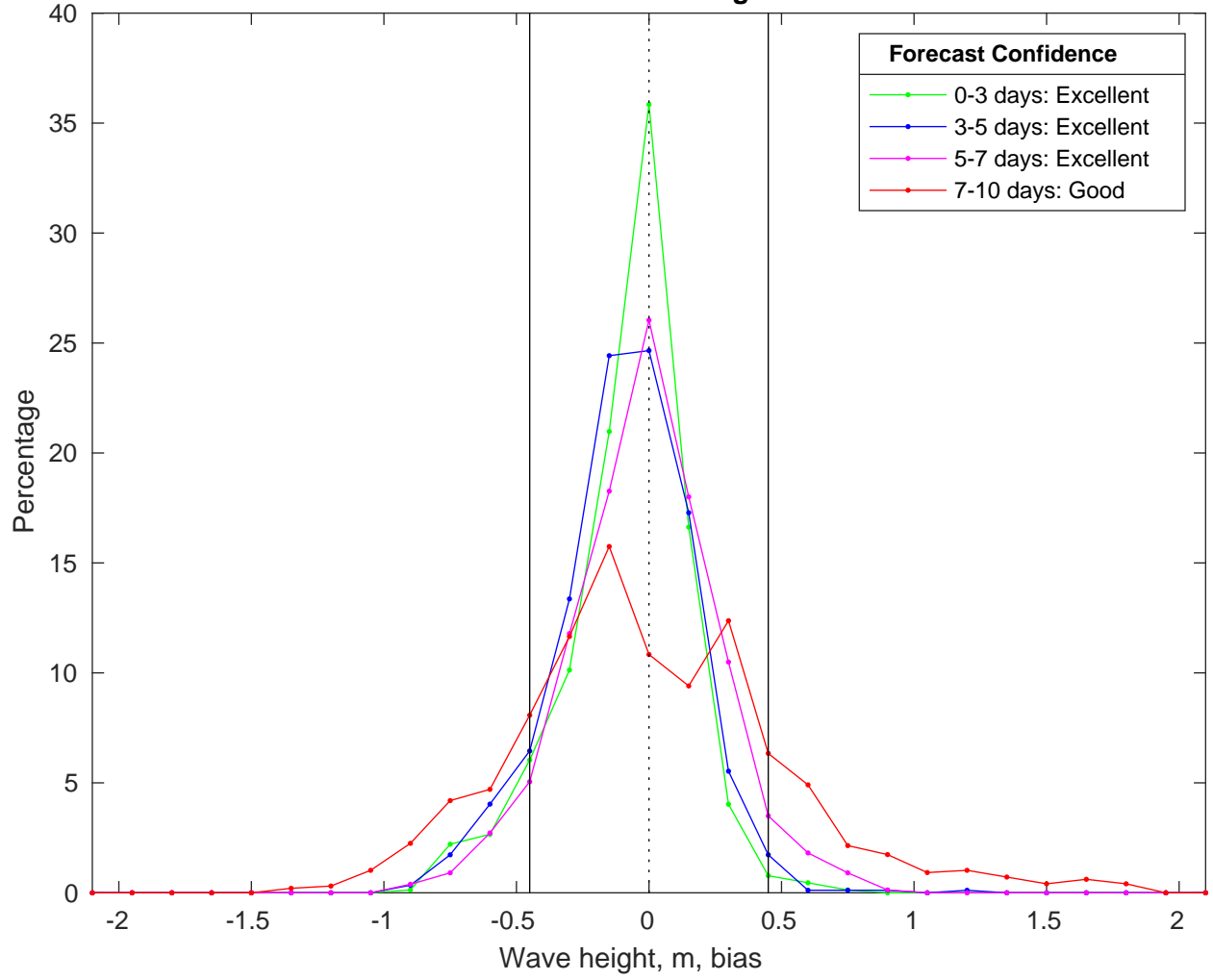
NDBC 41004 vs CMEMS Waves Bias Histogram: 29-Mar-2025
