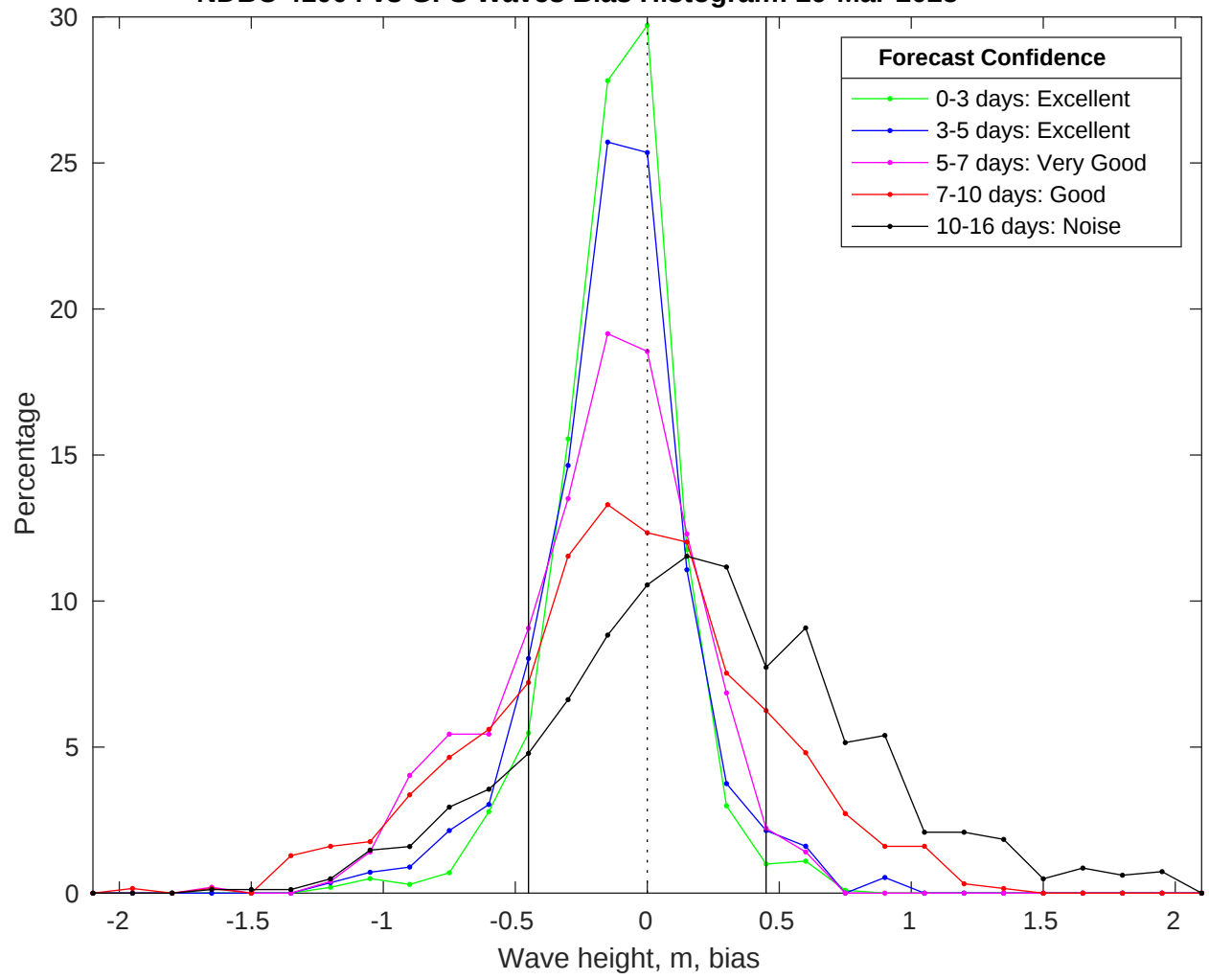
NDBC 41004 vs GFS Waves Bias Histogram: 29-Mar-2025
