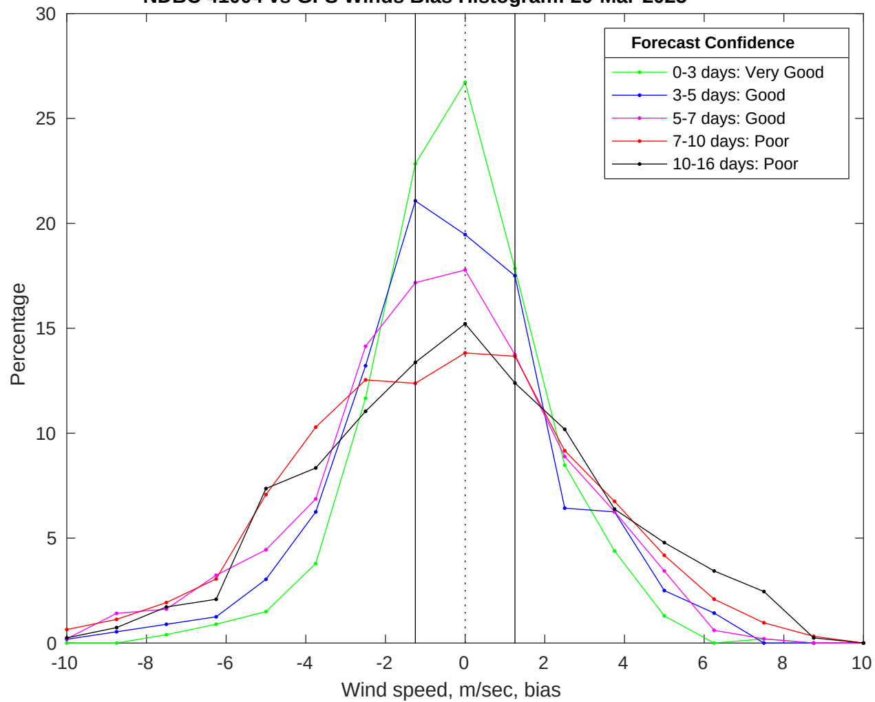
NDBC 41004 vs GFS Winds Bias Histogram: 29-Mar-2025
