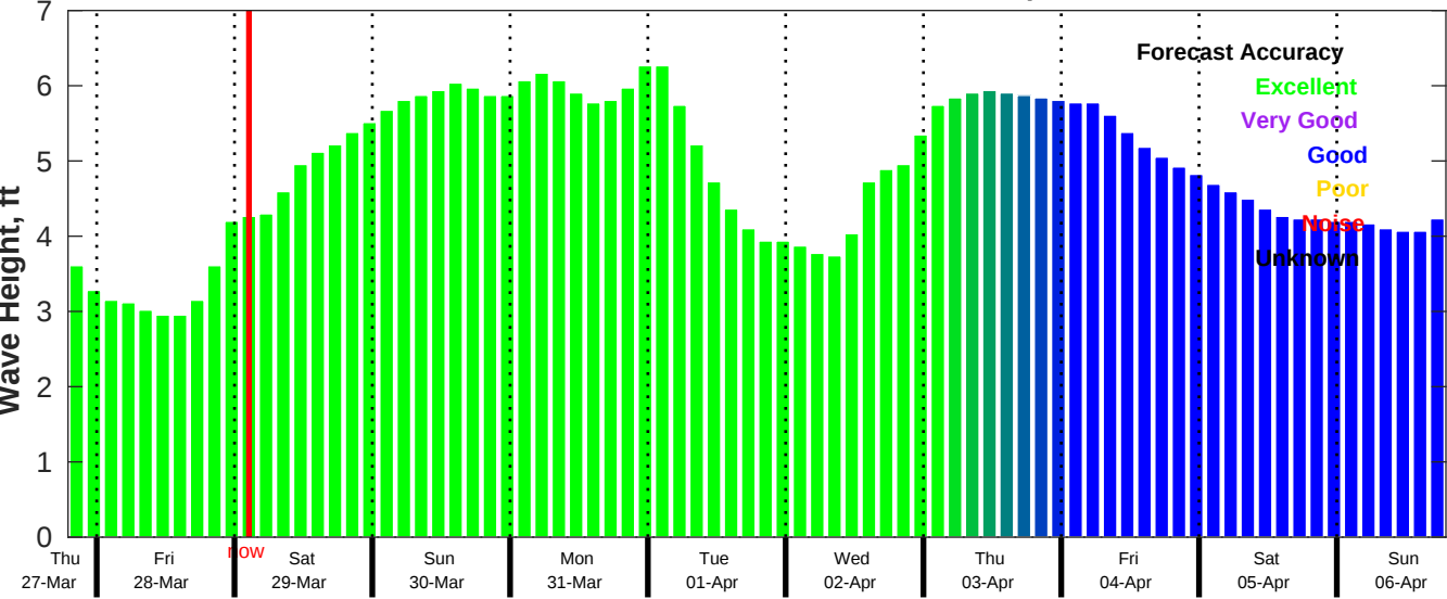
CMEMS Wave Forecast for NDBC 41004 from 27-Mar-2025 19:00:00 to 06-Apr-2025 19:00:00
