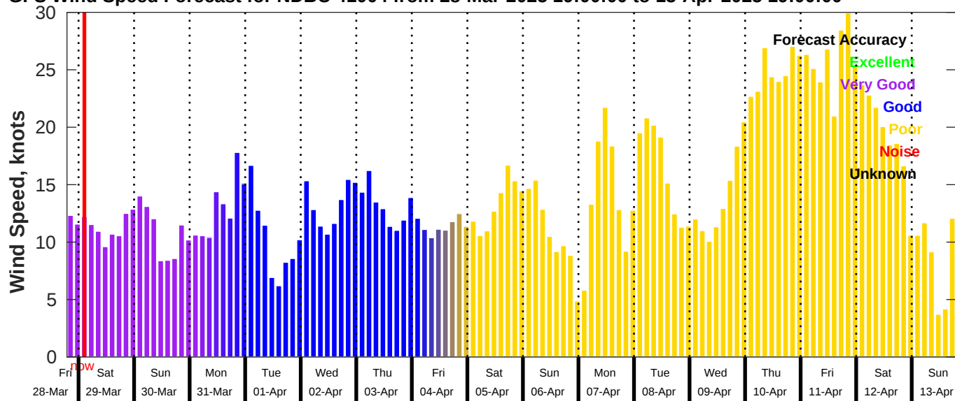
GFS Wind Speed Forecast for NDBC 41004 from 28-Mar-2025 19:00:00 to 13-Apr-2025 19:00:00
