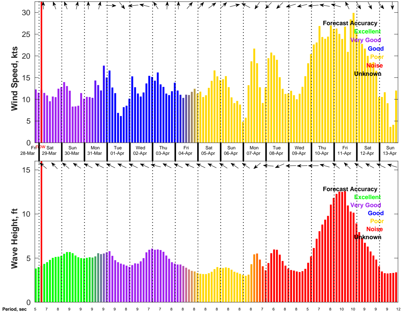
Wind & Wave Forecast for NDBC 41004 from 28-Mar-2025 19:00:00 to 13-Apr-2025 19:00:00
