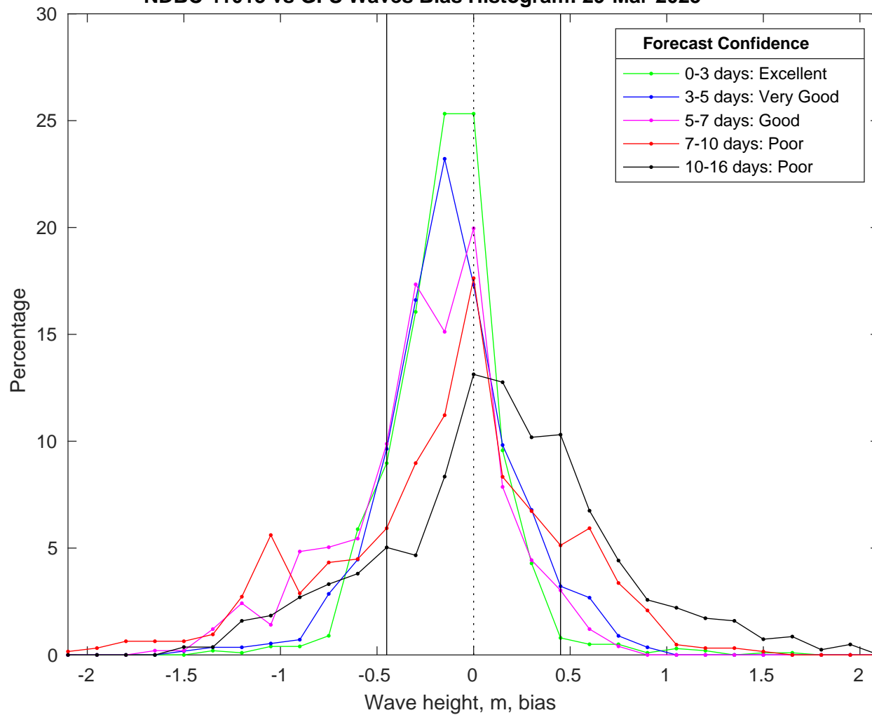
NDBC 41013 vs GFS Waves Bias Histogram: 29-Mar-2025
