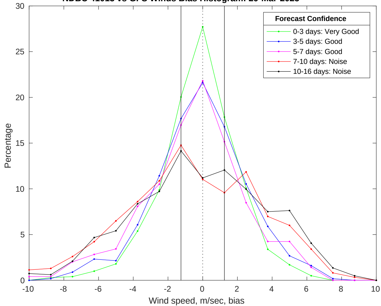
NDBC 41013 vs GFS Winds Bias Histogram: 29-Mar-2025
