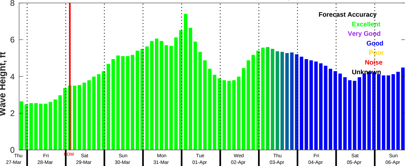
CMEMS Wave Forecast for NDBC 41013 from 27-Mar-2025 19:00:00 to 06-Apr-2025 19:00:00
