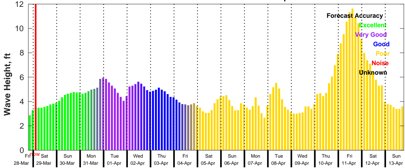
GFS Wave Forecast for NDBC 41013 from 28-Mar-2025 19:00:00 to 13-Apr-2025 19:00:00
