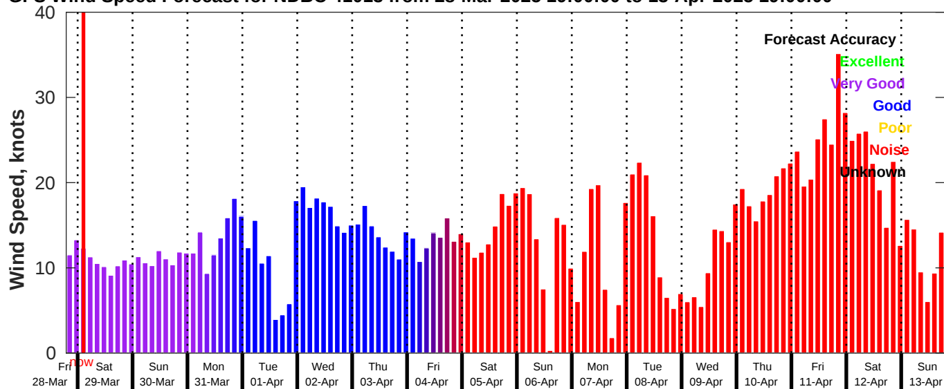
GFS Wind Speed Forecast for NDBC 41013 from 28-Mar-2025 19:00:00 to 13-Apr-2025 19:00:00
