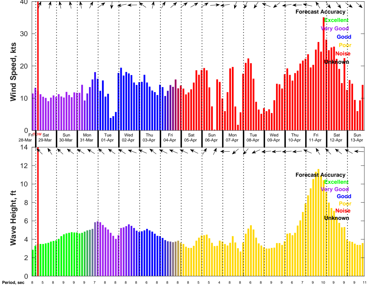
Wind & Wave Forecast for NDBC 41013 from 28-Mar-2025 19:00:00 to 13-Apr-2025 19:00:00
