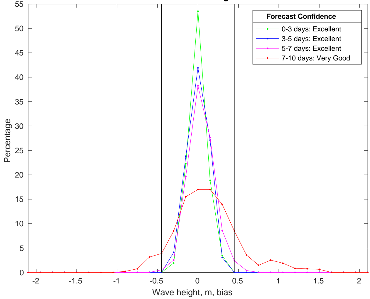
NDBC 41040 vs CMEMS Waves Bias Histogram: 29-Mar-2025
