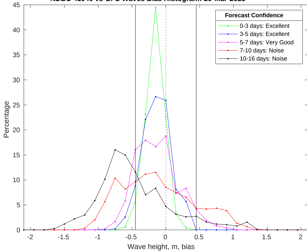
NDBC 41040 vs GFS Waves Bias Histogram: 29-Mar-2025
