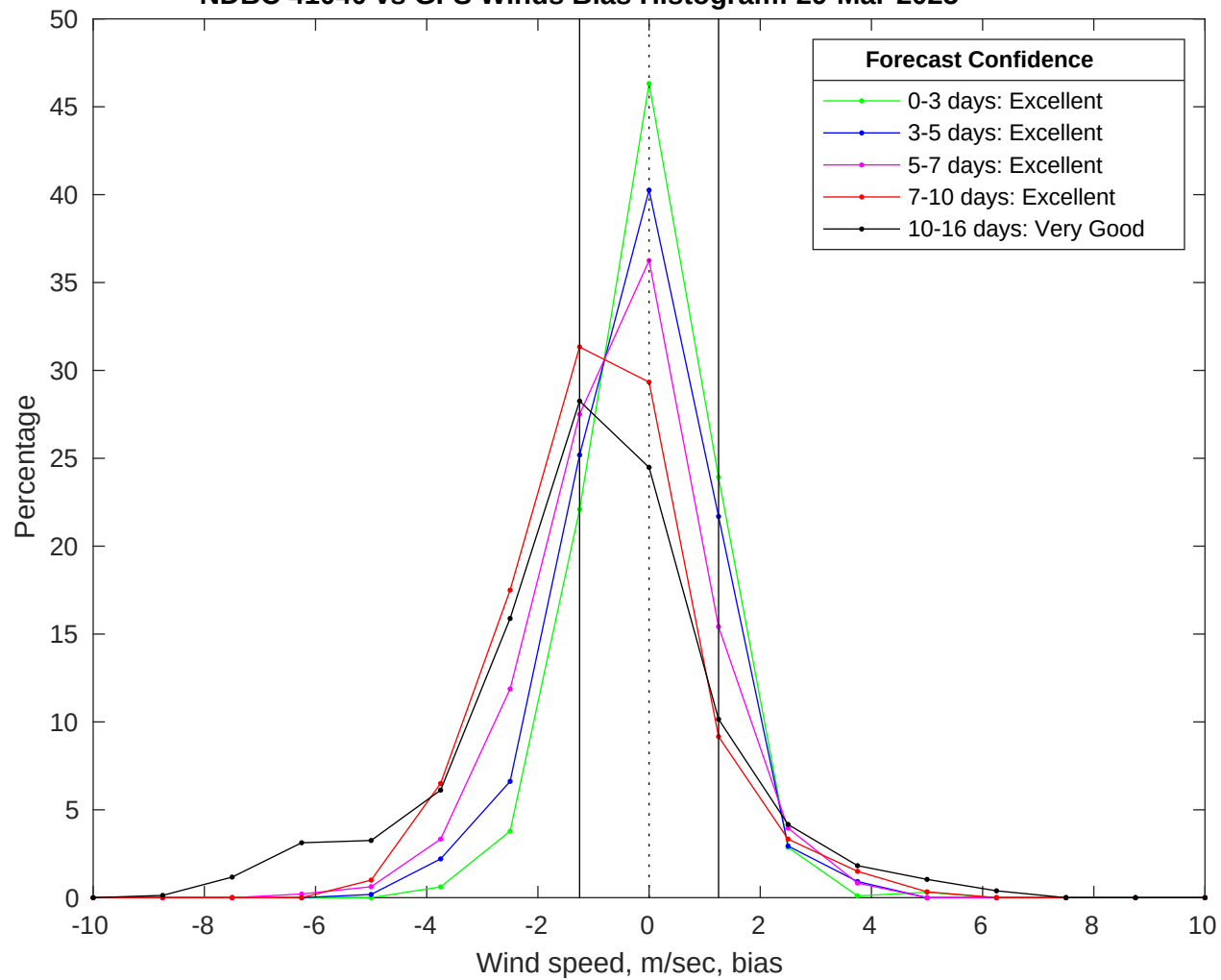
NDBC 41040 vs GFS Winds Bias Histogram: 29-Mar-2025
