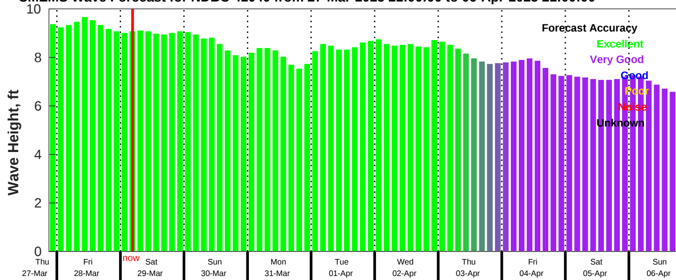
CMEMS Wave Forecast for NDBC 41040 from 27-Mar-2025 21:00:00 to 06-Apr-2025 21:00:00
