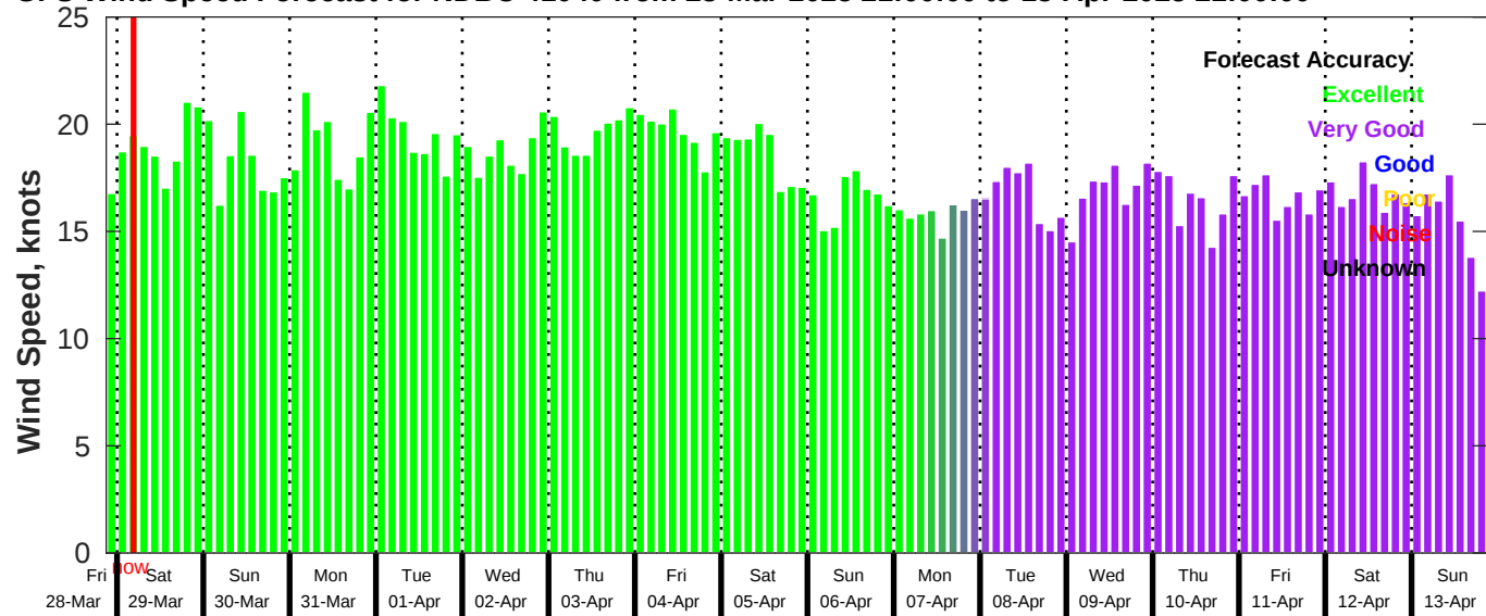
GFS Wind Speed Forecast for NDBC 41040 from 28-Mar-2025 21:00:00 to 13-Apr-2025 21:00:00
