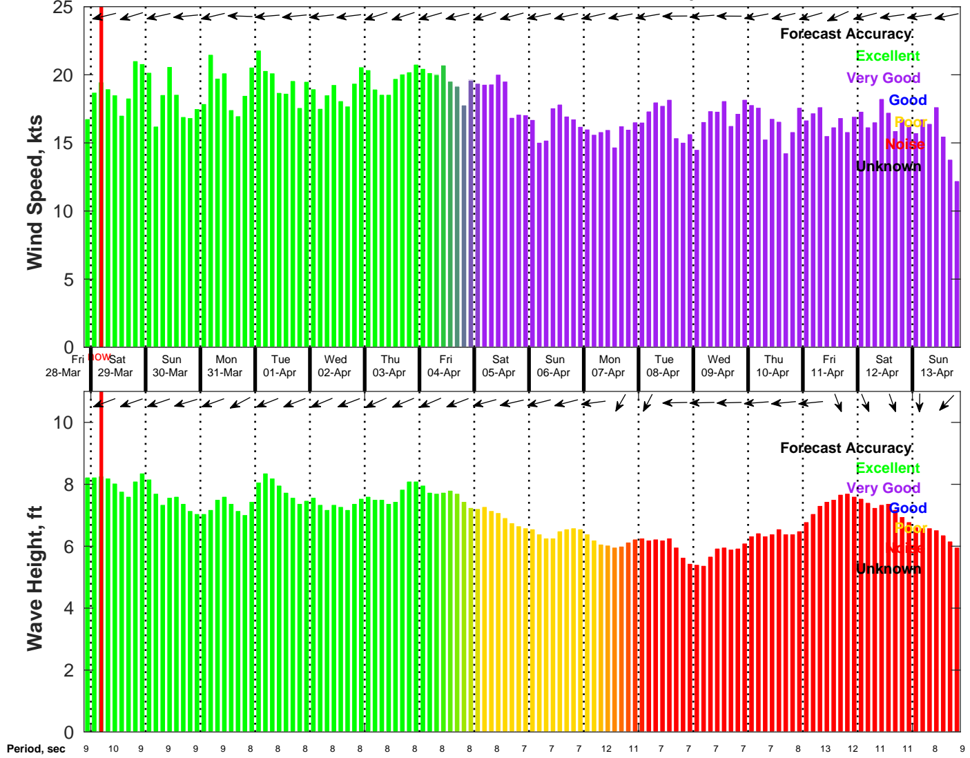
Wind & Wave Forecast for NDBC 41040 from 28-Mar-2025 21:00:00 to 13-Apr-2025 21:00:00
