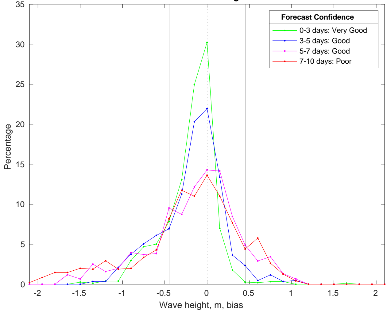
NDBC 42019 vs CMEMS Waves Bias Histogram: 29-Mar-2025
