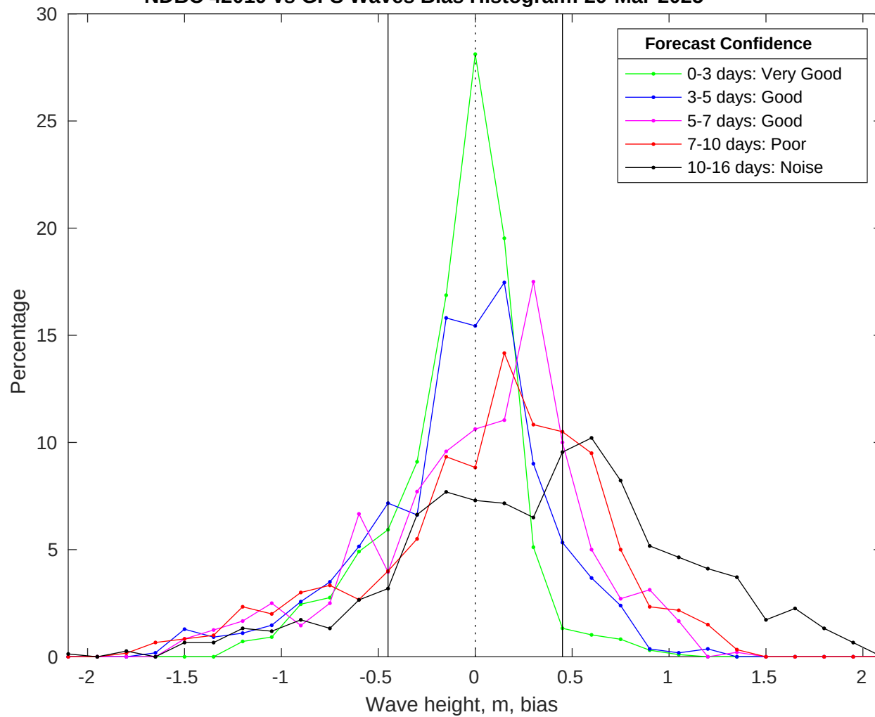
NDBC 42019 vs GFS Waves Bias Histogram: 29-Mar-2025
