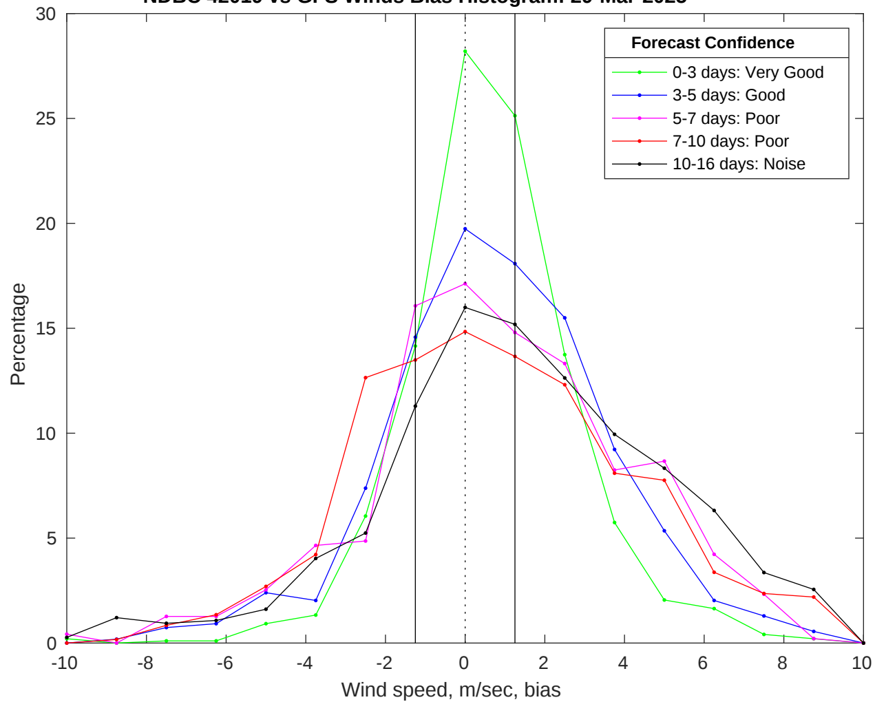
NDBC 42019 vs GFS Winds Bias Histogram: 29-Mar-2025
