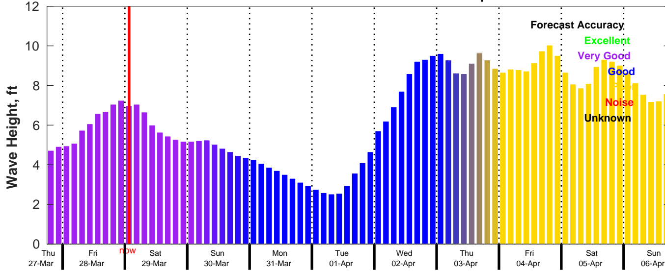
CMEMS Wave Forecast for NDBC 42019 from 27-Mar-2025 18:00:00 to 06-Apr-2025 18:00:00
