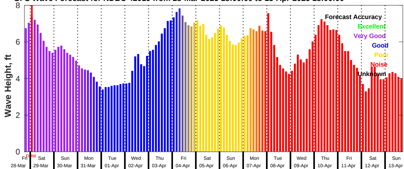
GFS Wave Forecast for NDBC 42019 from 28-Mar-2025 18:00:00 to 13-Apr-2025 18:00:00
