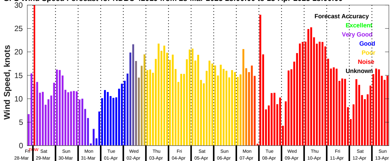
GFS Wind Speed Forecast for NDBC 42019 from 28-Mar-2025 18:00:00 to 13-Apr-2025 18:00:00
