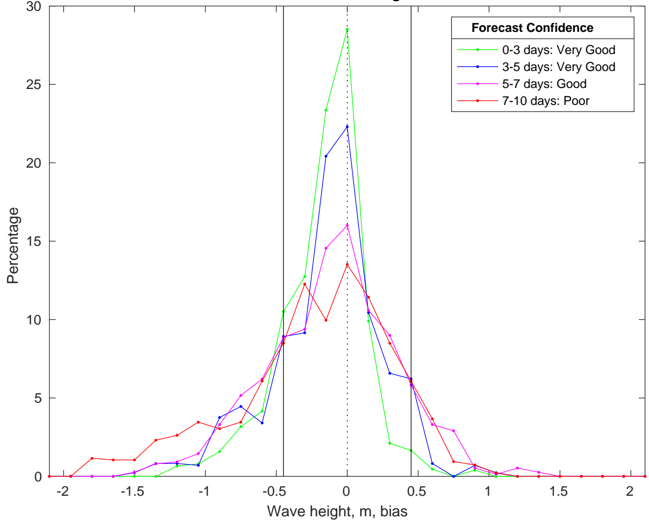
NDBC 42020 vs CMEMS Waves Bias Histogram: 29-Mar-2025
