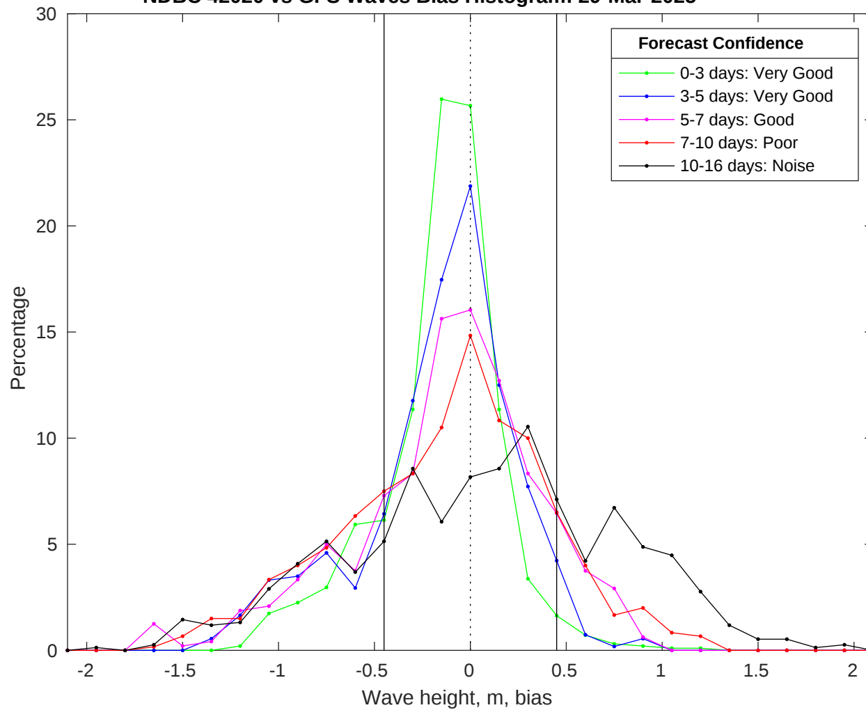
NDBC 42020 vs GFS Waves Bias Histogram: 29-Mar-2025
