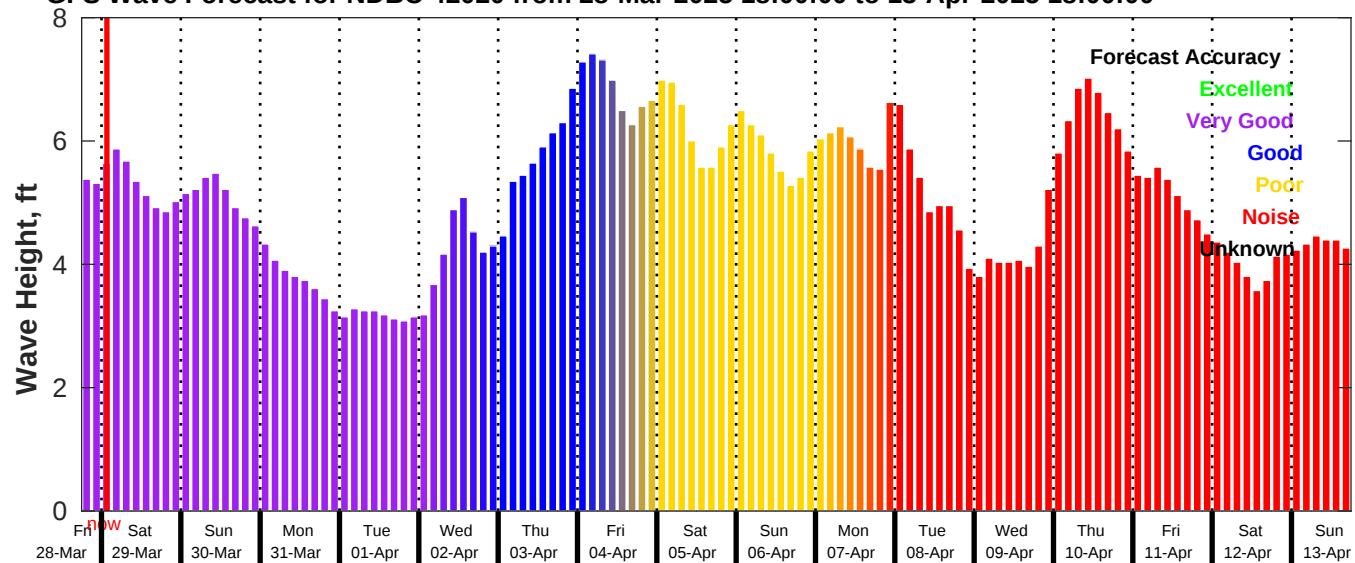
GFS Wave Forecast for NDBC 42020 from 28-Mar-2025 18:00:00 to 13-Apr-2025 18:00:00
