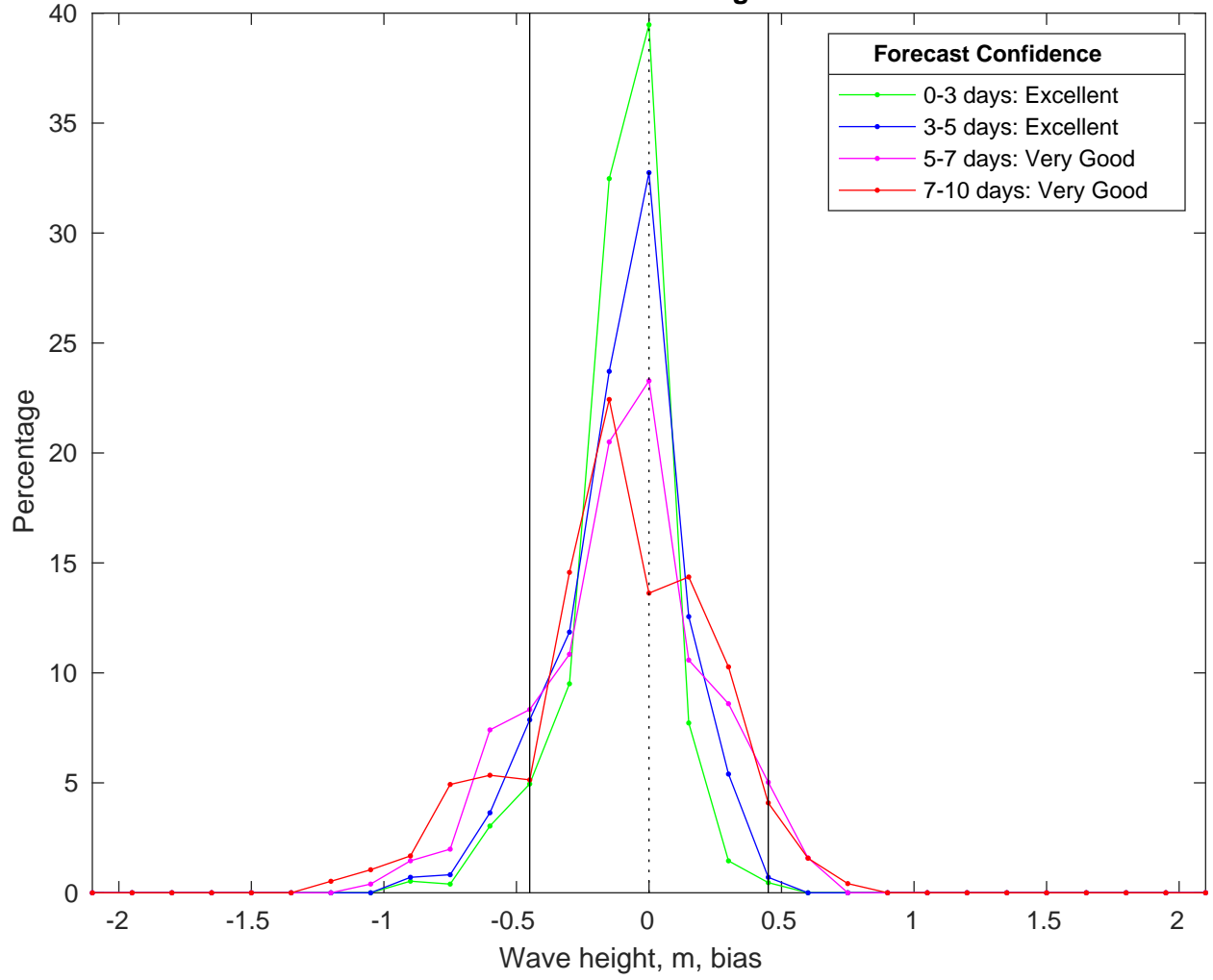
NDBC 42035 vs CMEMS Waves Bias Histogram: 29-Mar-2025
