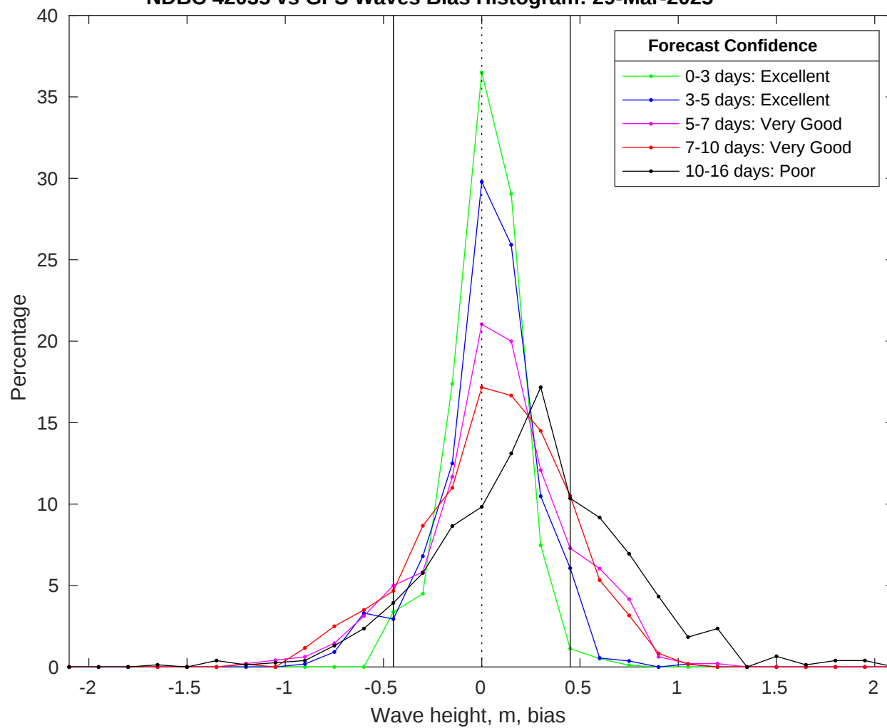
NDBC 42035 vs GFS Waves Bias Histogram: 29-Mar-2025
