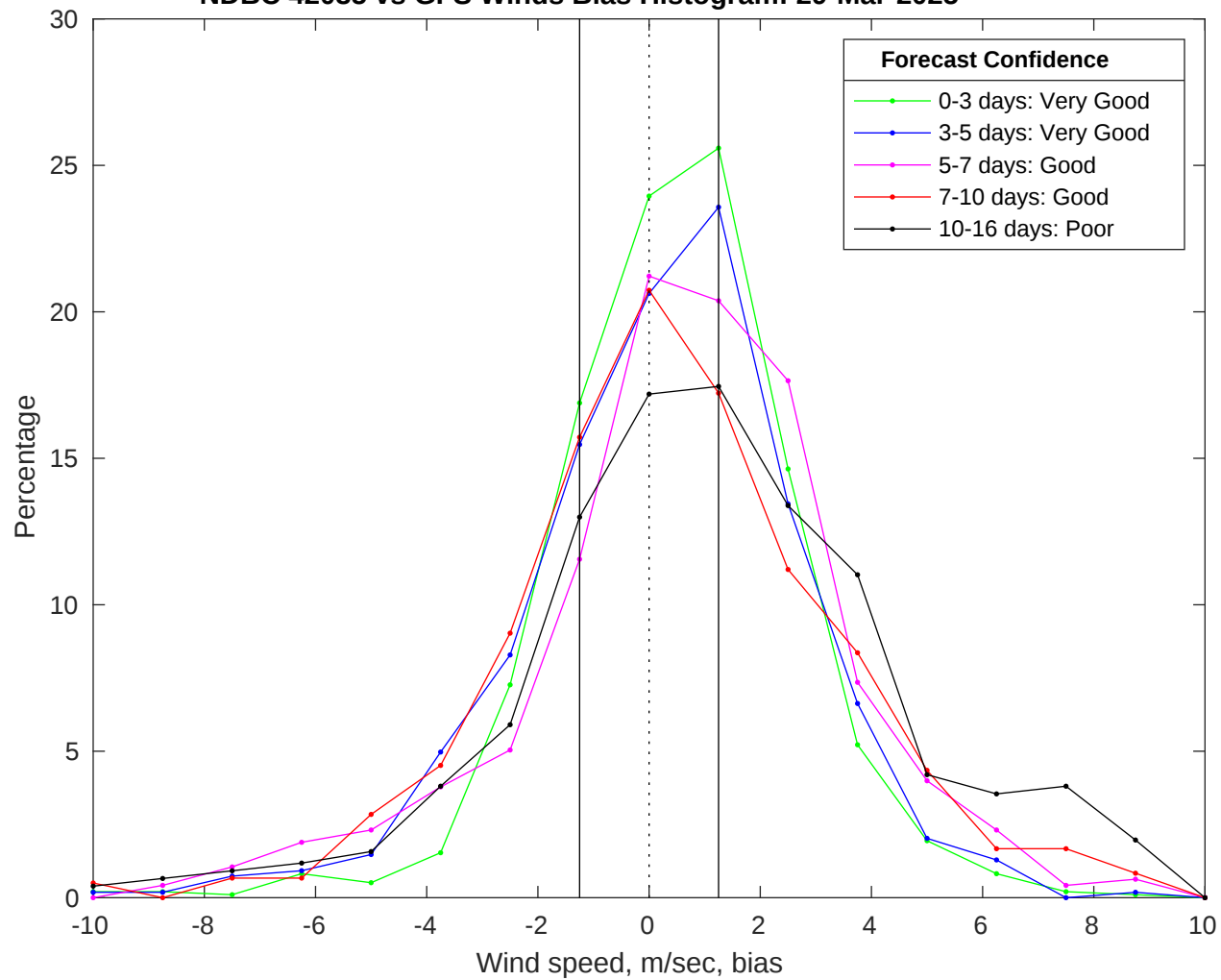
NDBC 42035 vs GFS Winds Bias Histogram: 29-Mar-2025
