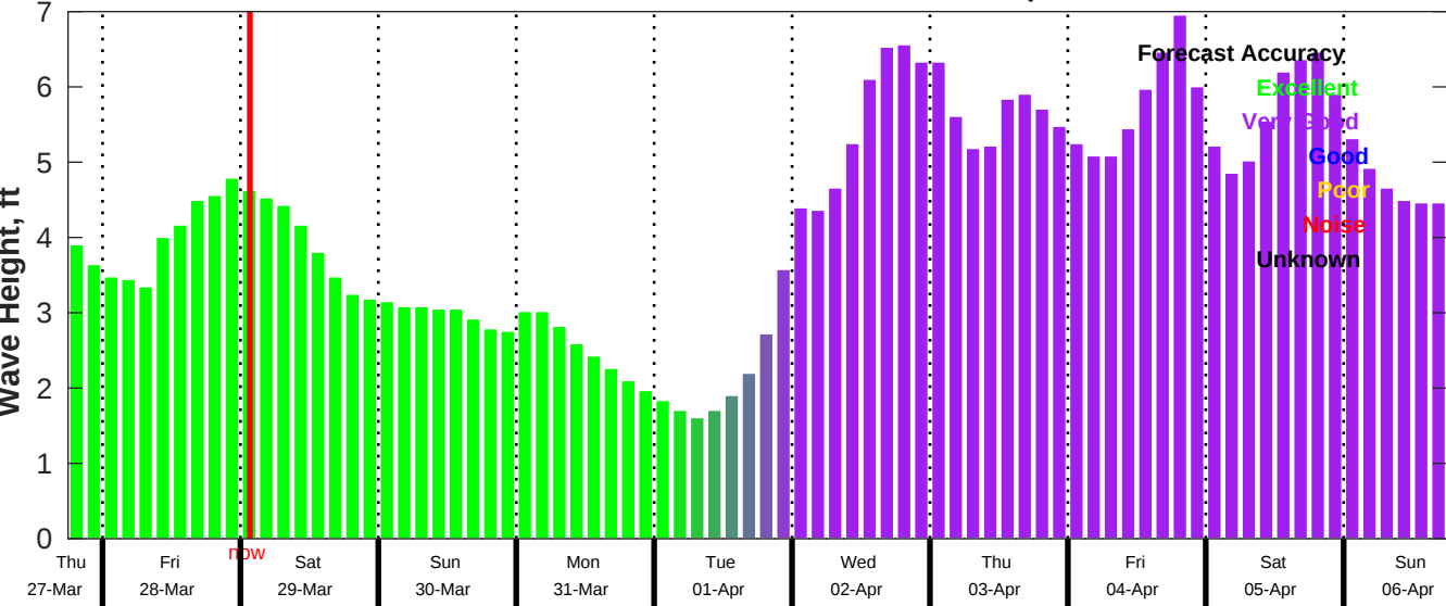
CMEMS Wave Forecast for NDBC 42035 from 27-Mar-2025 18:00:00 to 06-Apr-2025 18:00:00
