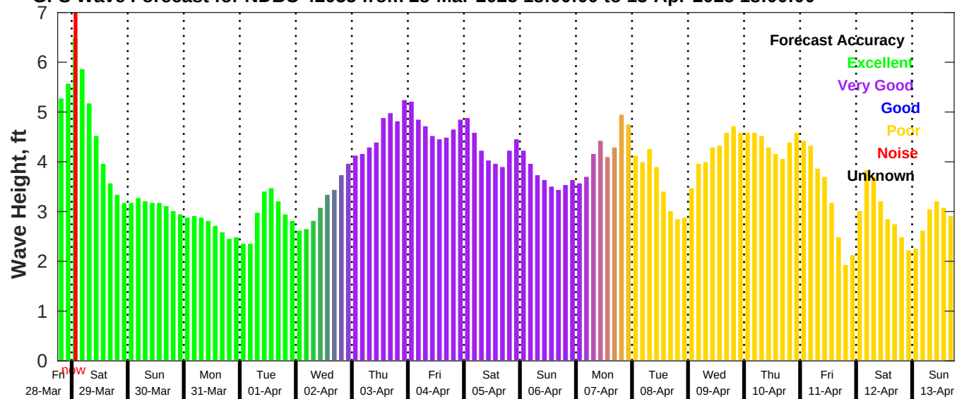
GFS Wave Forecast for NDBC 42035 from 28-Mar-2025 18:00:00 to 13-Apr-2025 18:00:00
