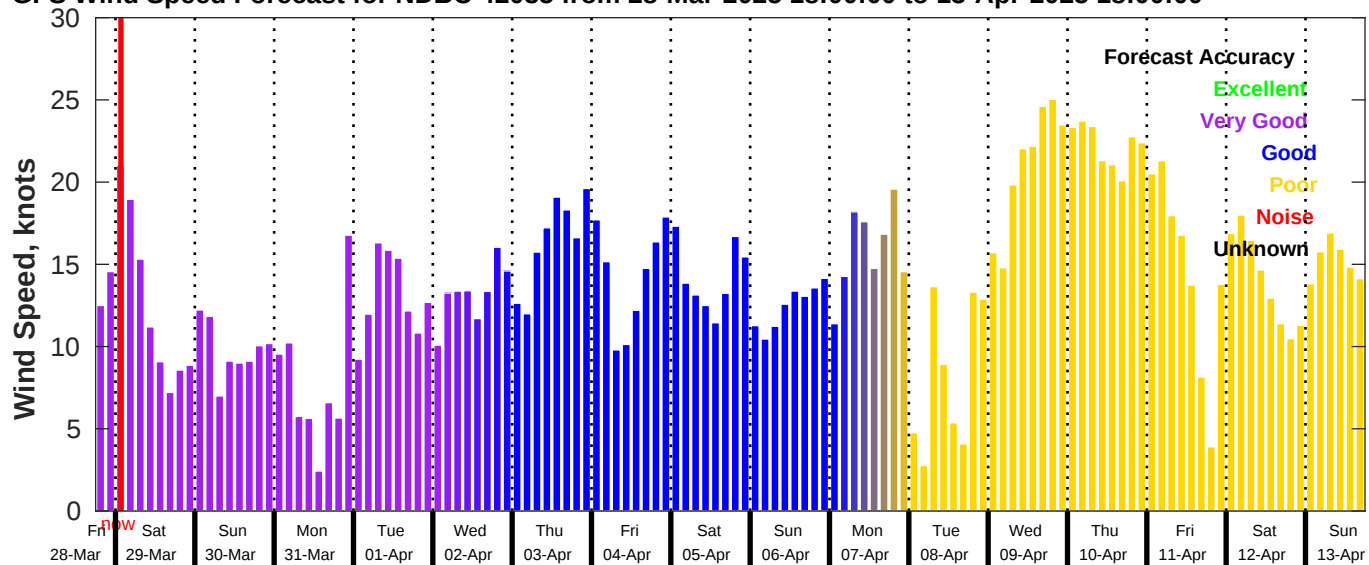
GFS Wind Speed Forecast for NDBC 42035 from 28-Mar-2025 18:00:00 to 13-Apr-2025 18:00:00
