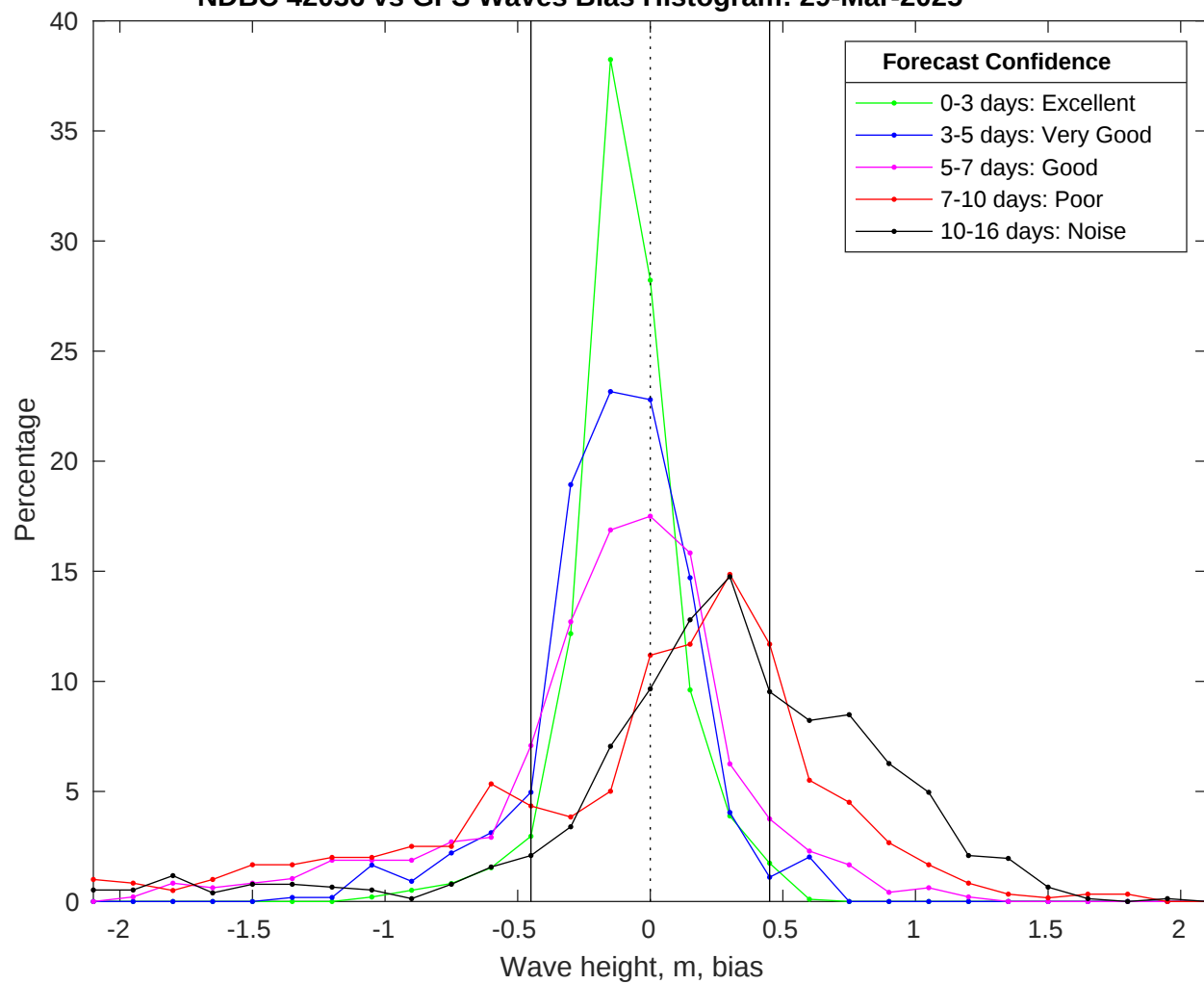
NDBC 42036 vs GFS Waves Bias Histogram: 29-Mar-2025
