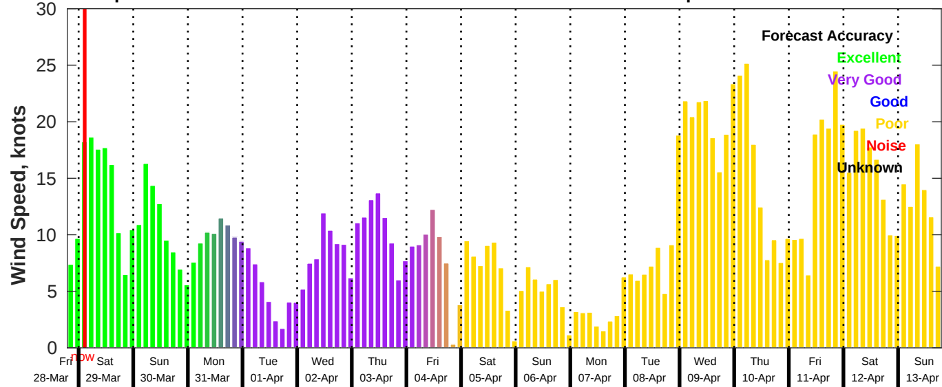
GFS Wind Speed Forecast for NDBC 42036 from 28-Mar-2025 19:00:00 to 13-Apr-2025 19:00:00
