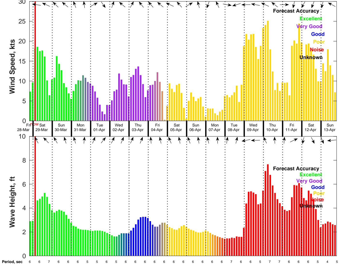
Wind & Wave Forecast for NDBC 42036 from 28-Mar-2025 19:00:00 to 13-Apr-2025 19:00:00
