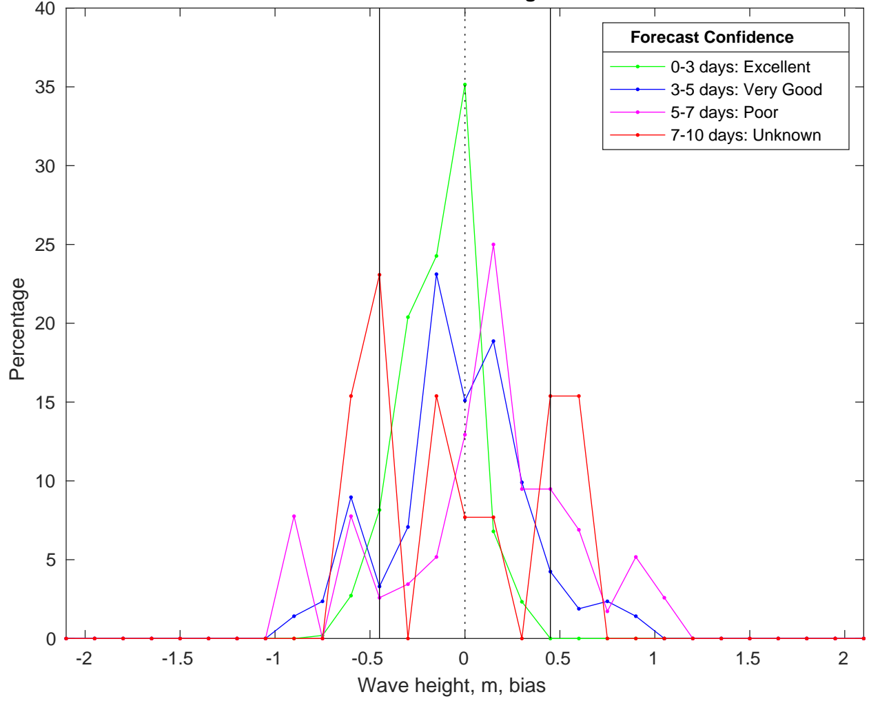
NDBC 42040 vs CMEMS Waves Bias Histogram: 29-Mar-2025
