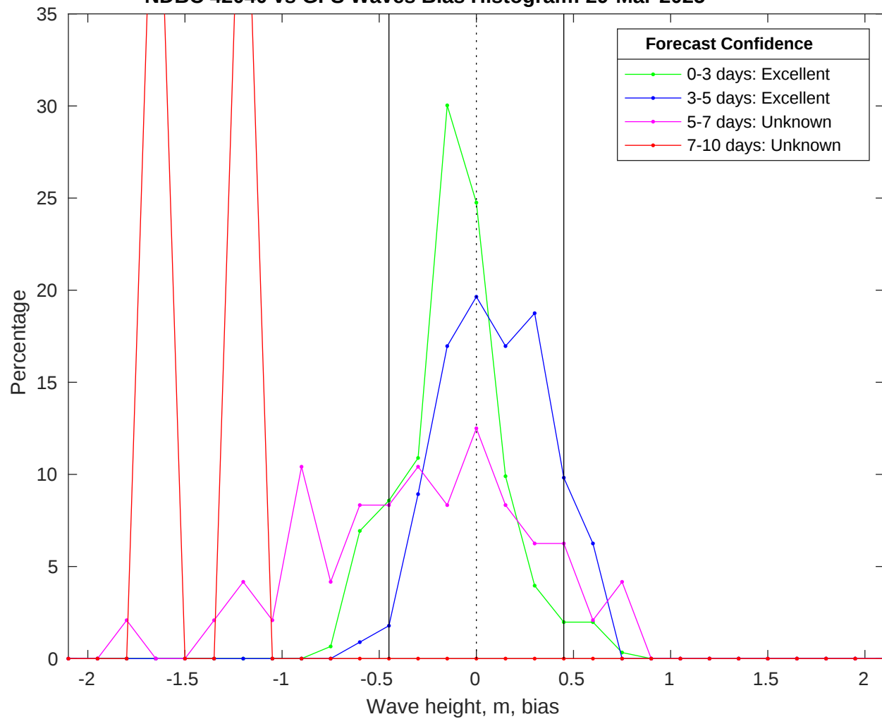
NDBC 42040 vs GFS Waves Bias Histogram: 29-Mar-2025
