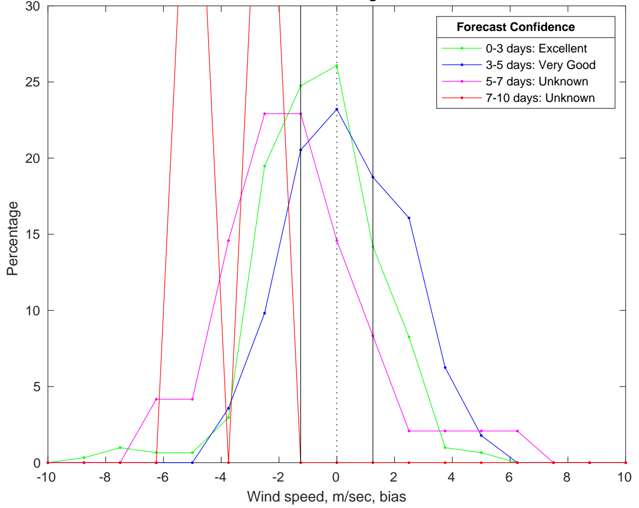
NDBC 42040 vs GFS Winds Bias Histogram: 29-Mar-2025
