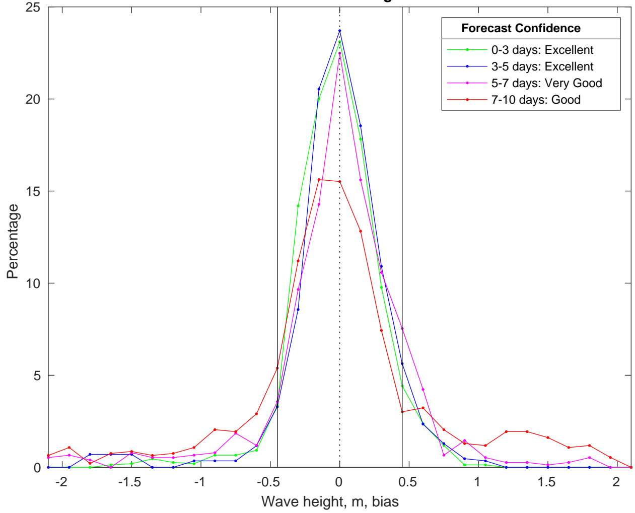
NDBC 46011 vs CMEMS Waves Bias Histogram: 29-Mar-2025
