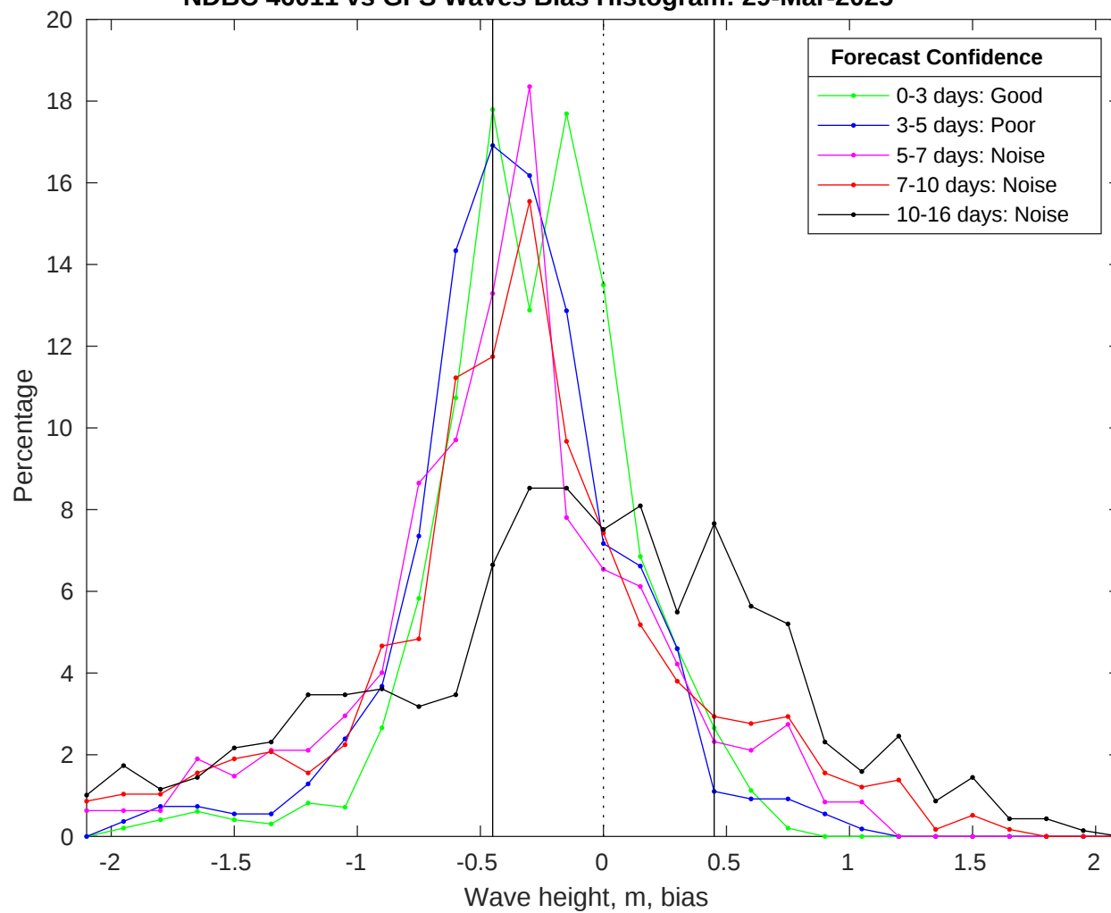
NDBC 46011 vs GFS Waves Bias Histogram: 29-Mar-2025
