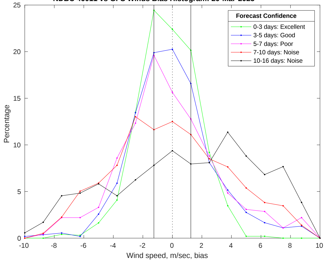
NDBC 46011 vs GFS Winds Bias Histogram: 29-Mar-2025
