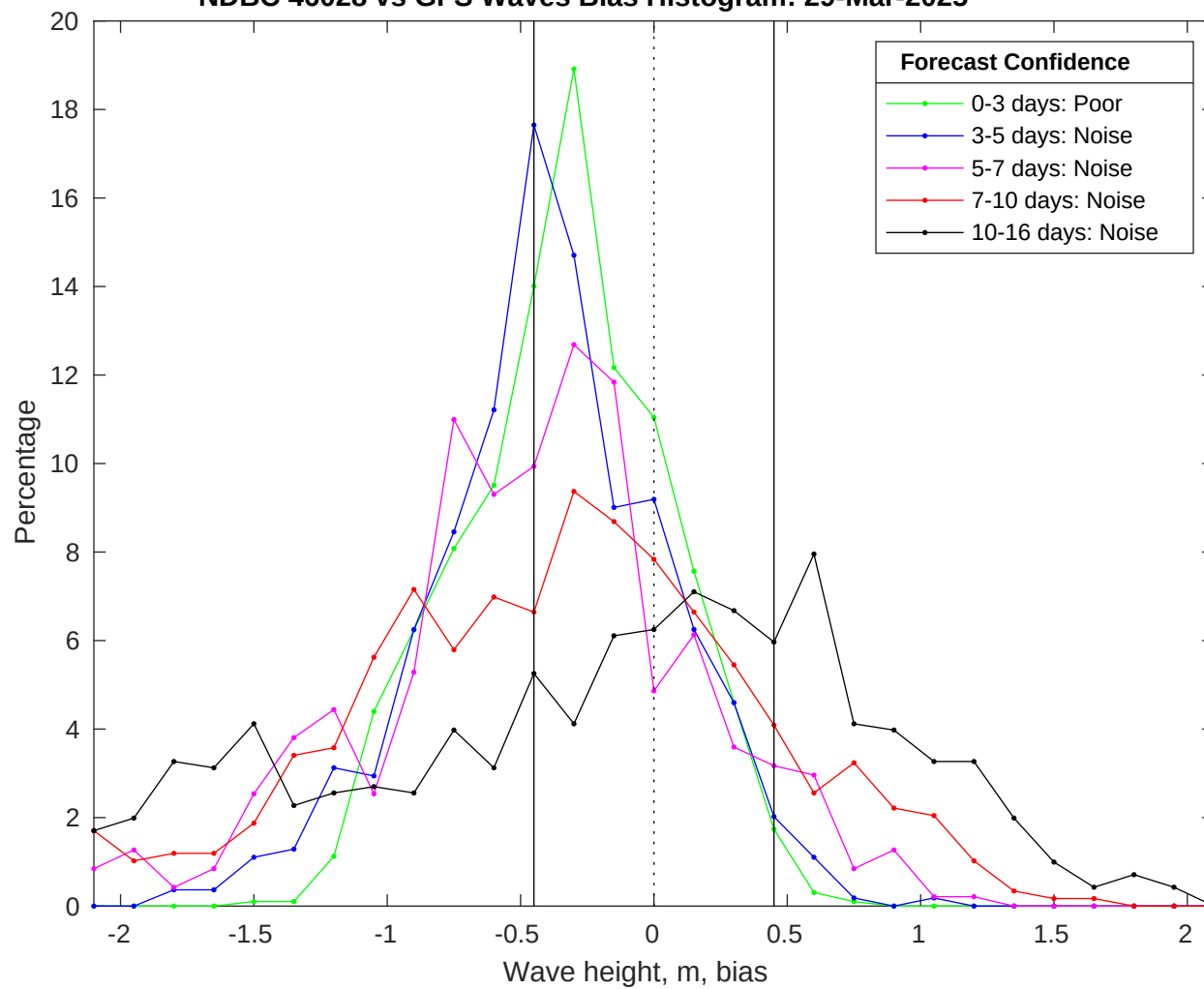
NDBC 46028 vs GFS Waves Bias Histogram: 29-Mar-2025
