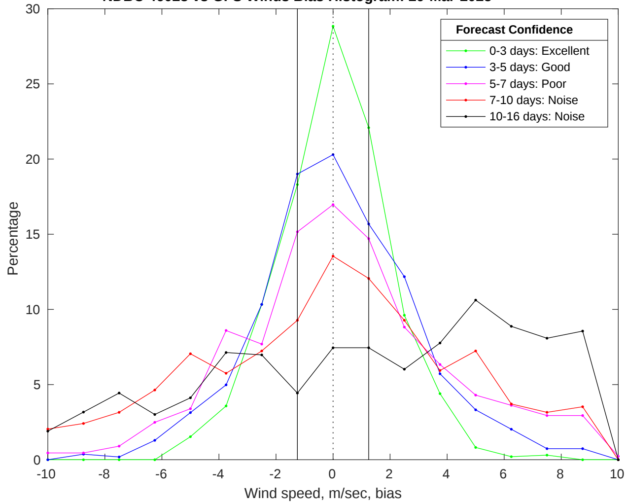
NDBC 46028 vs GFS Winds Bias Histogram: 29-Mar-2025
