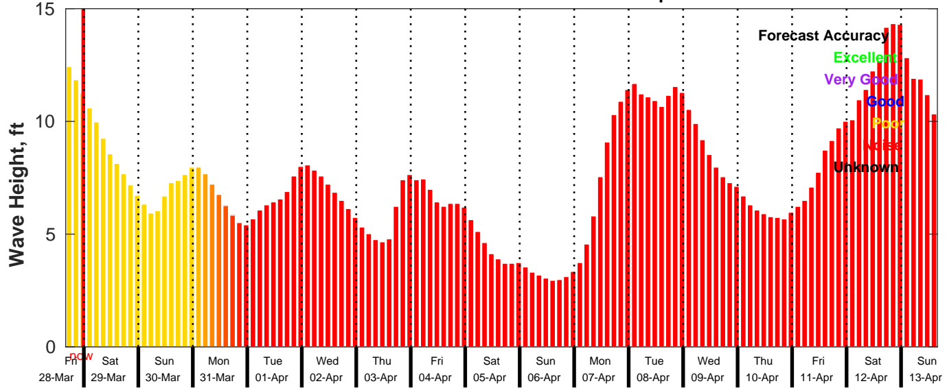
GFS Wave Forecast for NDBC 46028 from 28-Mar-2025 16:00:00 to 13-Apr-2025 16:00:00
