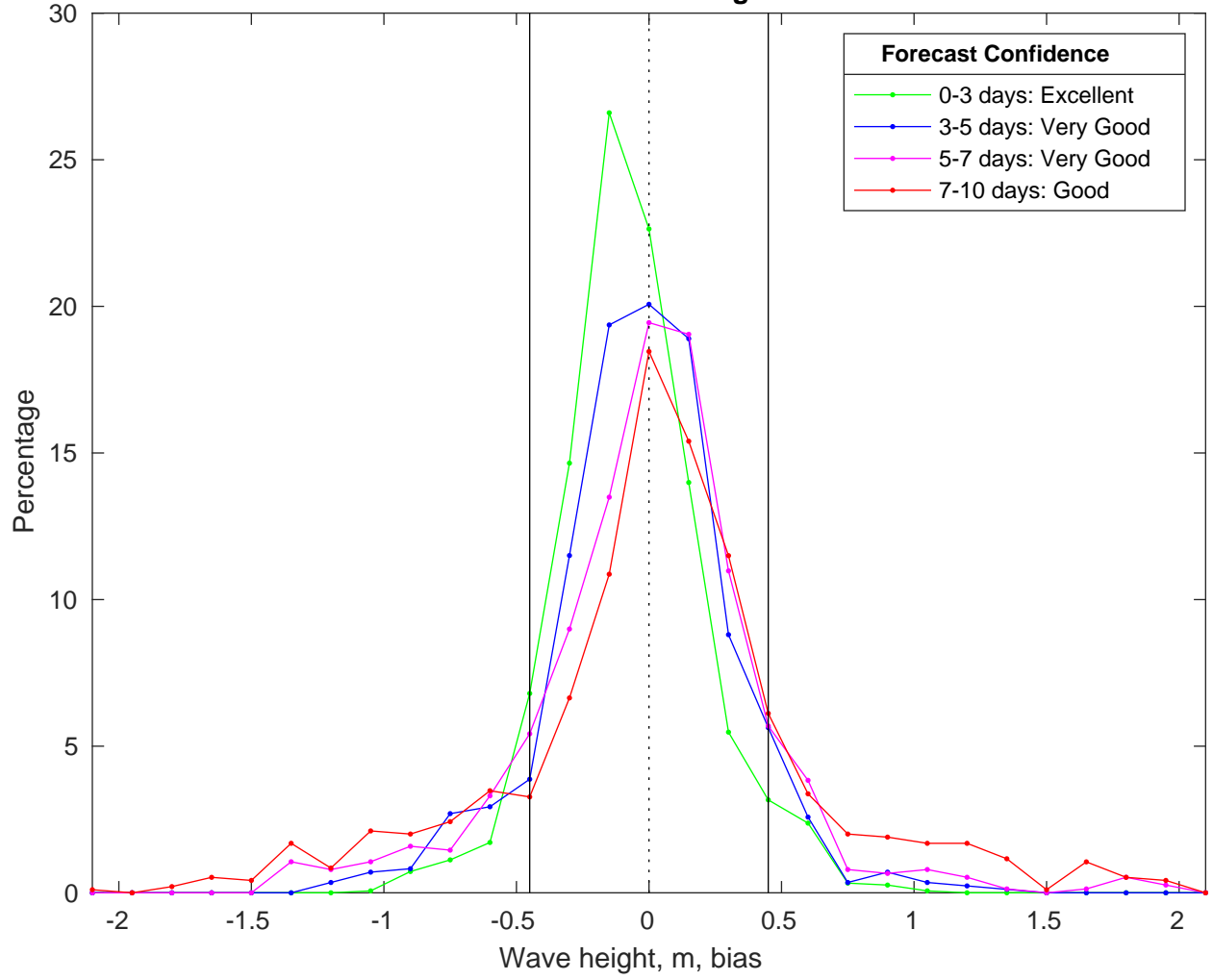
NDBC 46054 vs CMEMS Waves Bias Histogram: 29-Mar-2025
