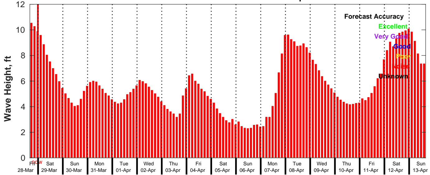
GFS Wave Forecast for NDBC 46054 from 28-Mar-2025 16:00:00 to 13-Apr-2025 16:00:00
