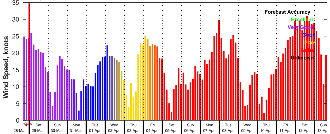
GFS Wind Speed Forecast for NDBC 46054 from 28-Mar-2025 16:00:00 to 13-Apr-2025 16:00:00
