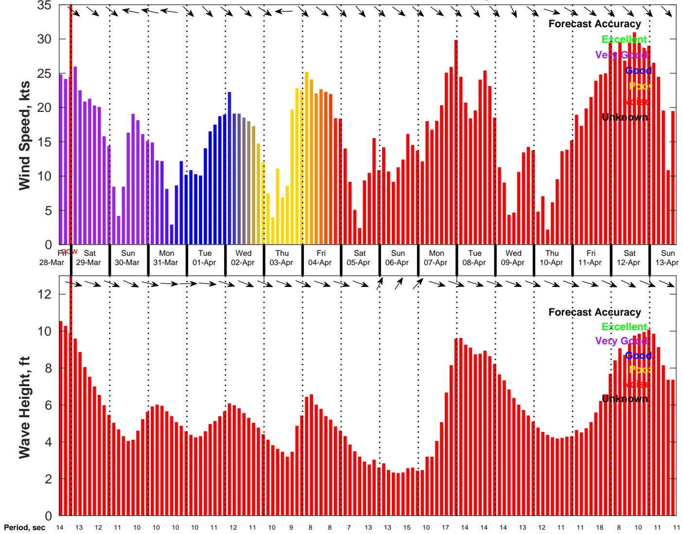
Wind & Wave Forecast for NDBC 46054 from 28-Mar-2025 16:00:00 to 13-Apr-2025 16:00:00
